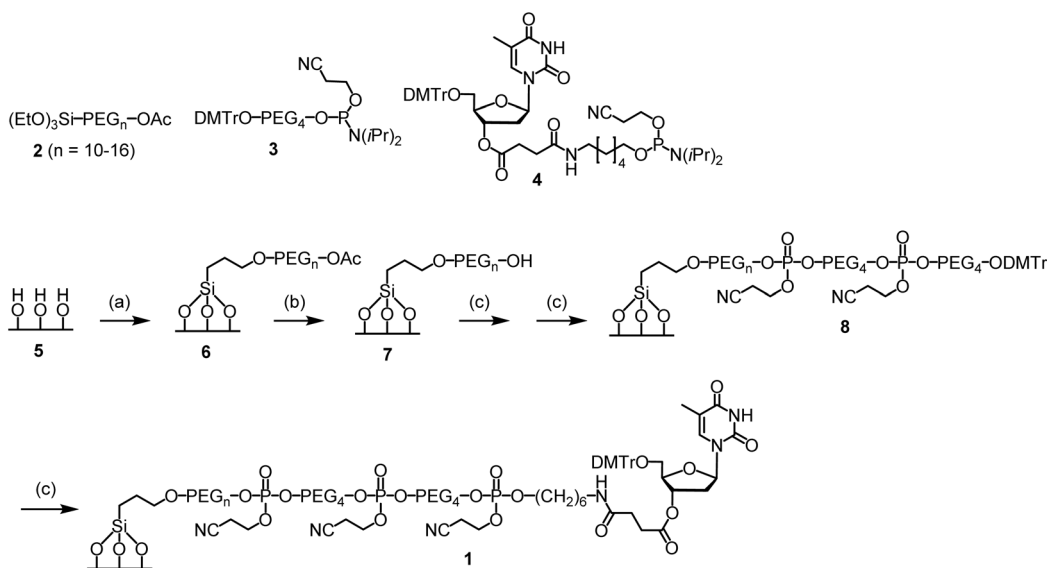
Scheme 2 Functionalization of glass wool and glass beads. Conditions: (a) 2 (1% PhMe), rt, 20 min; then, supernatant removed, glass wool 100 ° C, 4 h. (b) NH 4 OH (30%), 55 °C, 2 h. (c) On a DNA synthesizer, standard coupling, oxidation and deblocking conditions with modifications; see the ESI† for details.
