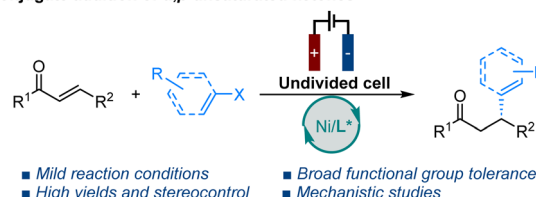
Scheme 1 Design of enantioselective electrochemical reductive conjugate addition.
