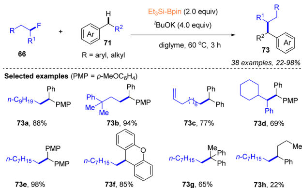
Scheme 25 Silylboronate-mediated cross-coupling of alkylfluorides and aryl alkanes.
