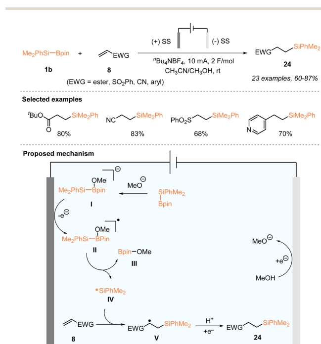
Scheme 8 Electrochemical hydrosilylation of alkenes with PhMe 2 Si-Bpin.
