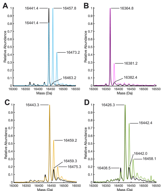
Fig. 3 Deconvoluted ESI TOF positive ion mode mass spectra of (A) 1 before (black) and after (blue) the addition of 10 equivalents of H 2 O 2 and incubation for 1 hour. (B) Deconvoluted mass spectra of 2 before (black) and after (pink) the addition of 10 equivalents of H 2 O 2 and incubation for 1 hour. (C) Deconvoluted mass spectra of 3 before (black) and after (yellow) the addition of 10 equivalents of H 2 O 2 and incubation for 1 hour. (D) Deconvoluted mass spectra of 4 before (black) and after (green) the addition of 10 equivalents of H 2 O 2 and incubation for 1 hour.
