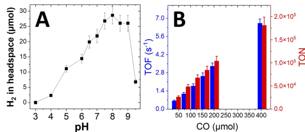
Fig. 5 (A) Quantity of H 2 in headspace of WGSR experiment determined by GC after 24 h versus pH (1 mL CO injected at t 0 ), 0.7 nmol per cm 2 Rec-RrCODH and 14 nmol per cm 2 NiPNP Arg , (buffer used: 50 mM citric acid pH 3, 50 mM sodium acetate pH 4 to 5.5, 50 mM Bis-Tris propane buffer pH 6 to 9.5); (B) turnover frequency (TOF) measured after 1 h WGSR, according to the total amount of Rec-RrCODH , and turnover number (TON) measured after 24 h versus starting amount of injected CO (50 mM Bis-Tris propane buffer pH 7, 0.9 nmol per cm 2 Rec-RrCODH and 110 nmol per cm 2 NiPNP Arg ).
