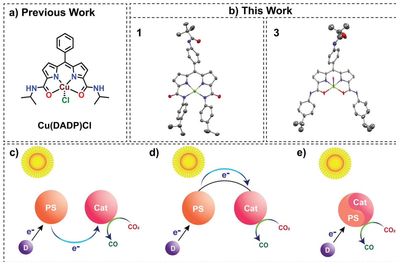
Fig. 1 (a) Previously reported literature on a similar diamidodipyrrin-based ligand. (b) This work on the Cu-based modified diamidodipyrrin complex shows the N 4 (1) (K(18-crown-6)) and N 2 O 2 (3) congeners in the perspective view of their crystal structures with 60% and 20% thermal ellipsoid probabilities, respectively. Hydrogen atoms, 18-crown-6, and the solvent molecules are omitted for clarity. Schematic illustration of photocatalytic systems for CO 2 reduction. (c) PS and Cat as distinct functional units. (d) PS and Cat linked (e) self-sensitized system. (PS: photosensitizer, Cat: catalyst, and D: sacrificial donor).
