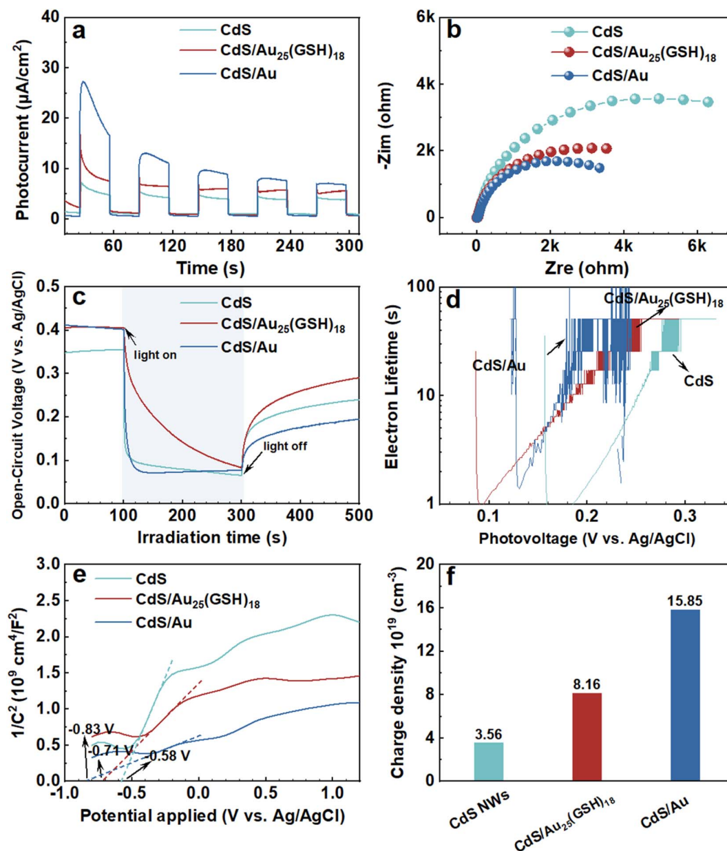
Fig. 5 PEC water splitting performances of CdS NWs, CdS/Au 25 (GSH) 18 and CdS/Au heterostructures in Na 2 SO 4 aqueous solution (pH = 6.69) under visible light irradiation ( \lambda > 420 \text{ nm} ) including (a) transient photocurrent responses (bias: 0.61 V vs. RHE), and (b) EIS results, (c) OCVD & (d) electron lifetime, and (e) Mott–Schottky plots & (f) charge carrier density ( N_D ).
