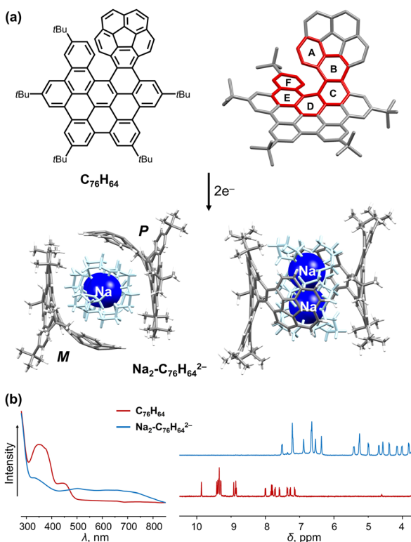
Fig. 1 (a) Structure of C_{76}H_{64} and chemical reduction to afford the dianion with Na^+ ions in top and side views. (b) Comparison of UV-vis absorption and ^1H NMR spectra of C_{76}H_{64} and its doubly-reduced product. 88,89
