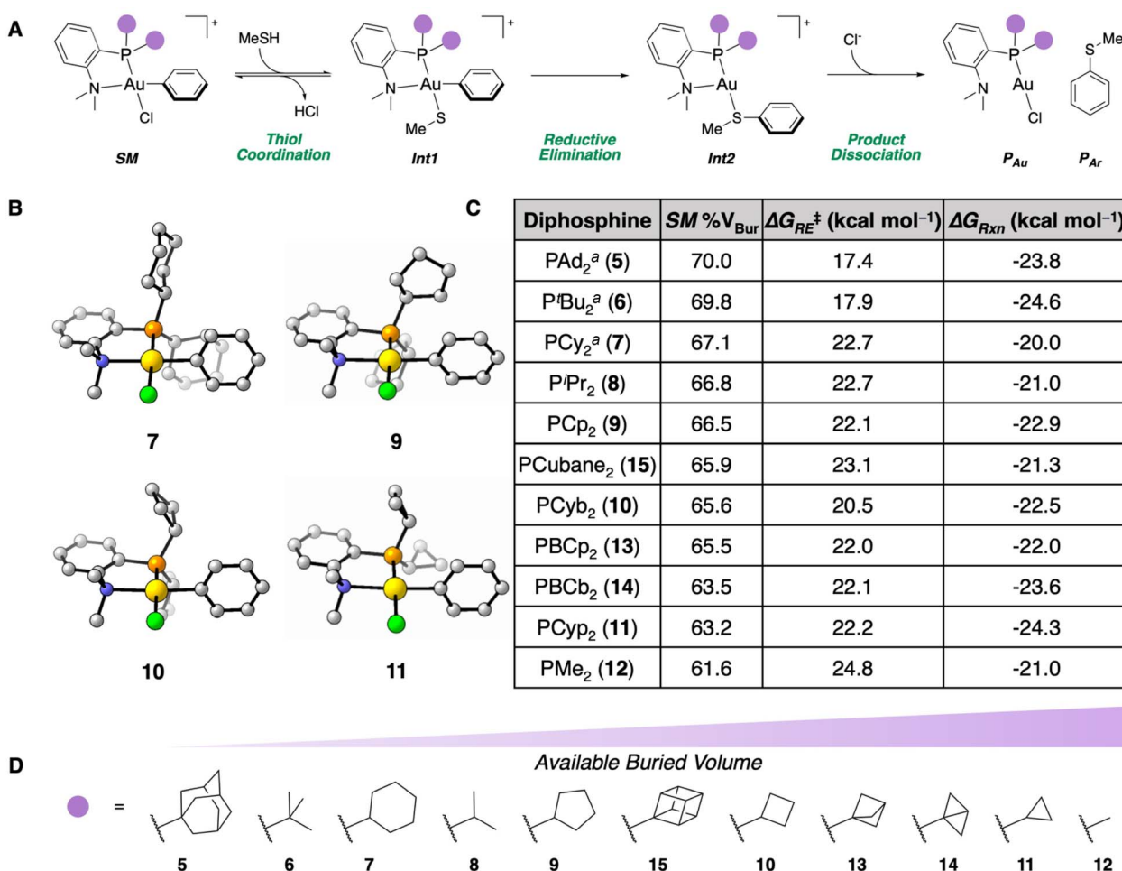
Fig. 2 (A) Proposed mechanism for the S -arylation of methanethiol mediated by Au(III) OACs. (B) SM geometries calculated for reagents 7 , 9 , 10 , and 11 at the \omega B97X-D/6-311+G(d,p), SDD, CPCM(water)//B3LYP-D3/6-31G(d), LANL2DZ, CPCM(water) level of theory. (C) Table of % V_{\text{Bur}} , \Delta G_{\text{RE}}^\ddagger , and \Delta G_{\text{Rxn}} for the different dialkylphosphine substituents examined. a These parameters were calculated previously. 35 (D) Schematic representation showing the dialkylphosphine variations in order of least to most available % V_{\text{Bur}} .
