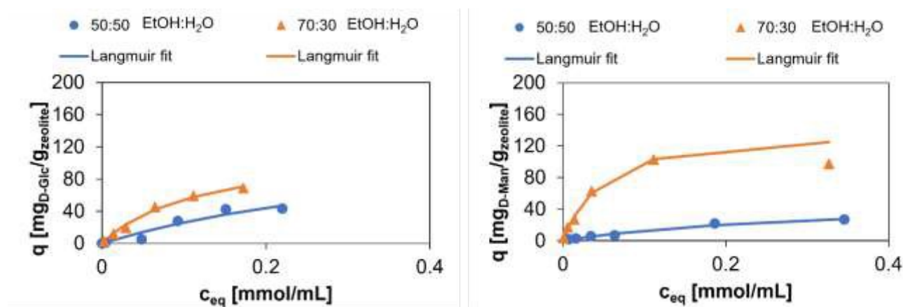
Figure 5. Adsorption isotherms for individually adsorbed D-Glc (left) and D-Man (right) on CaY zeolites at different EtOH:H 2 O ratios. Adsorption conditions: 500 mg zeolite, 3 mL EtOH:H 2 O solution, 2 h, RT, 500 rpm.
