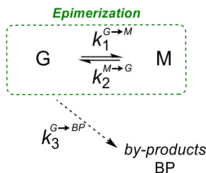
Figure 3. Proposed reaction network for D-Glc ( G ) epimerization to D-Man ( M ) catalyzed by Sn-OF-1.
