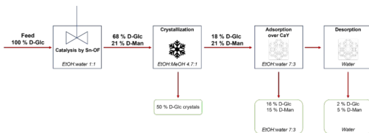
Figure 7. Synthesis and isolation of D-Man via epimerization of D-Glc in the presence of Sn-OF-1 followed by recovery of D-Man by adsorptive separation over CaY zeolite. Percent values reflect the carbon balance.
