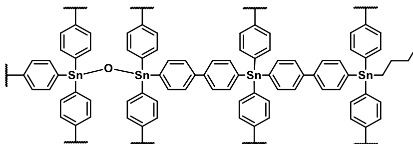
Figure 1. Structure of Sn-OF-1. 20
