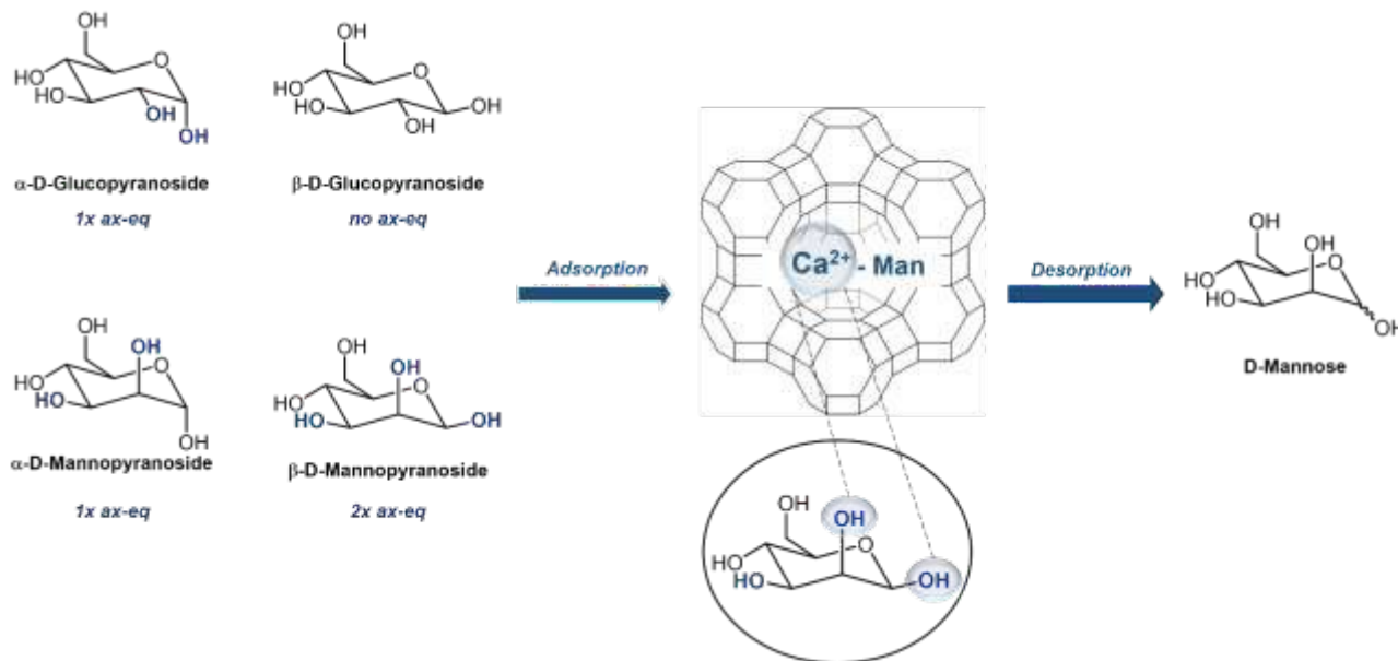
Figure 2. Separation of D-man via \text{Ca}^{2+} complexation in CaY zeolite.
