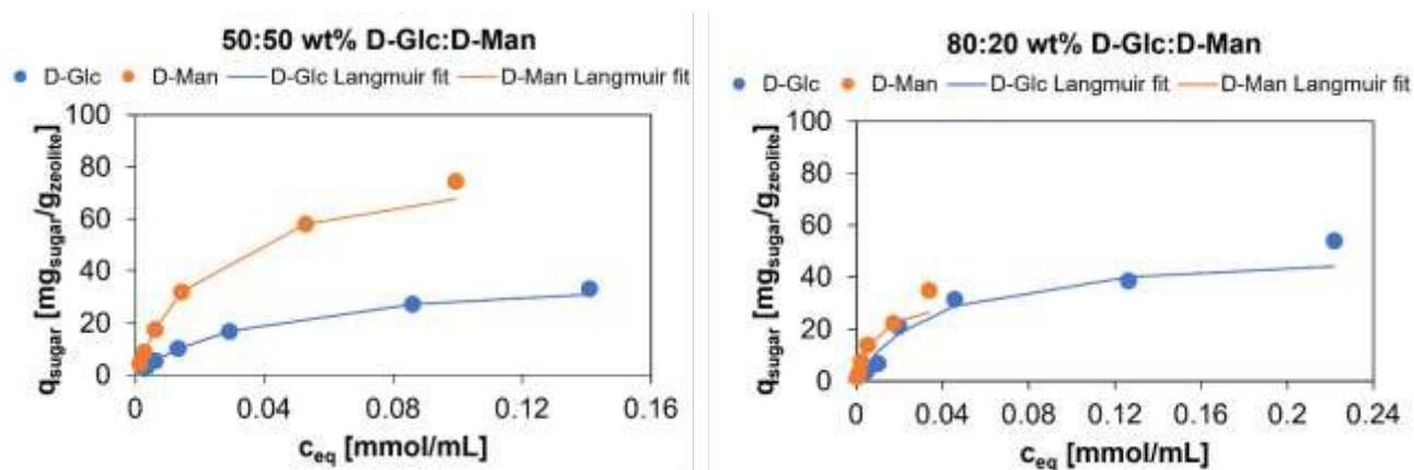
Figure 6. Competitive adsorption of D-Glc and D-Man by CaY zeolites. Adsorption conditions: 500 mg zeolite, 3 mL 70:30 wt% EtOH:H 2 O solution, 2 h, RT, 500 rpm.
