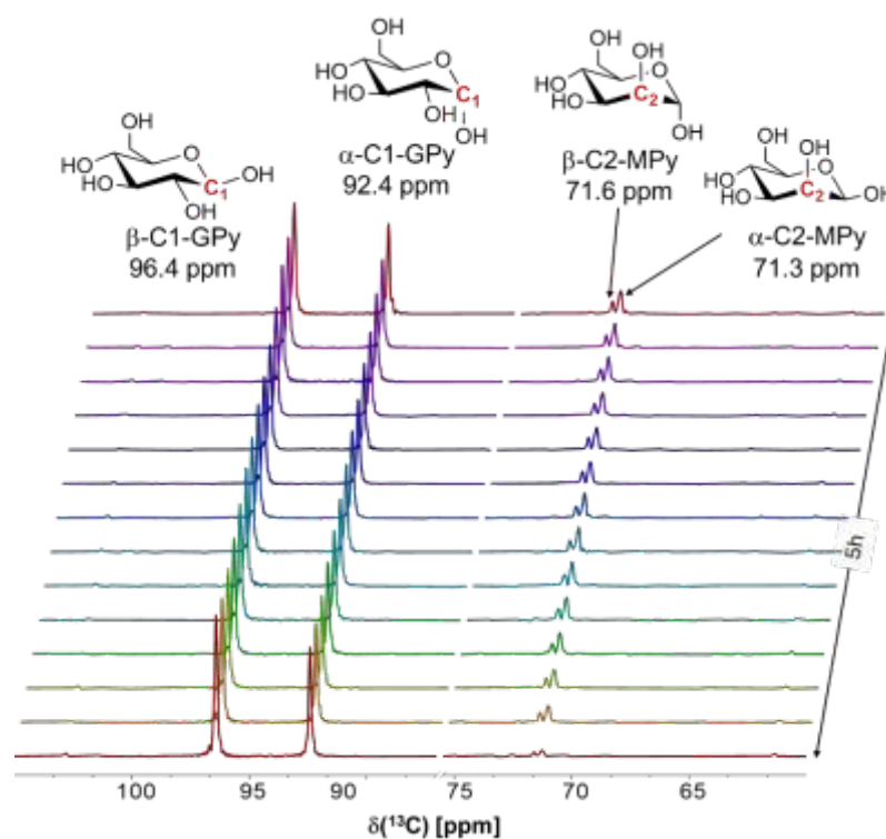
Figure 4. Direct polarization MAS solid-state ^{13}\text{C} NMR (11.7 T, 3 kHz MAS) of Sn-OF-1 (9.4 mg) in the presence of a solution of 1- ^{13}\text{C} -D-Glc in 50:50 wt% EtOH:H 2 O (7.0 mol·L -1 , 0.195 mL) at 92 °C. The time-resolved operando spectra show conversion of D-Glc to D-Man.
