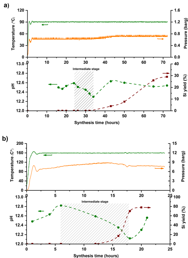
Fig. 2 Temperature, pressure, Si yield, and off-line pH profiles of MFI synthesis at (a) 90 and (b) 160 °C in FB reactor. Molar composition of the synthesis mixtures: 1 SiO_2 :0.5 TPAOH:20 H_2O from TEOS as Si-precursor. The dashed line only serves as a guide to the eye. At some points, extra pH measurements without yield extrapolation were done to fully map the synthesis.
