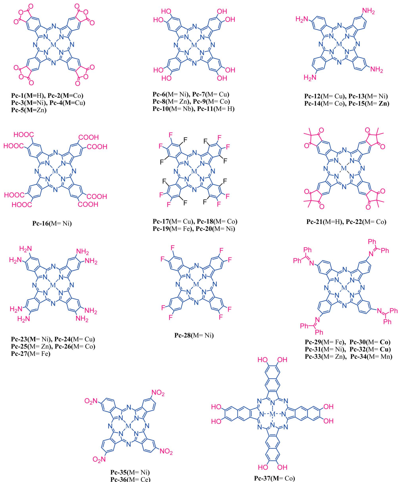
Fig. 3 Phthalocyanine building blocks reported.
