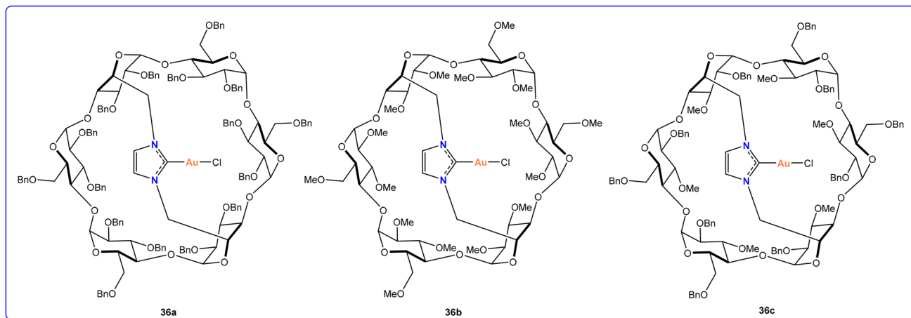
Scheme 15 (α-ICyD)-NHC-gold-catalyzed enantioselective cycloisomerization of enynes.
