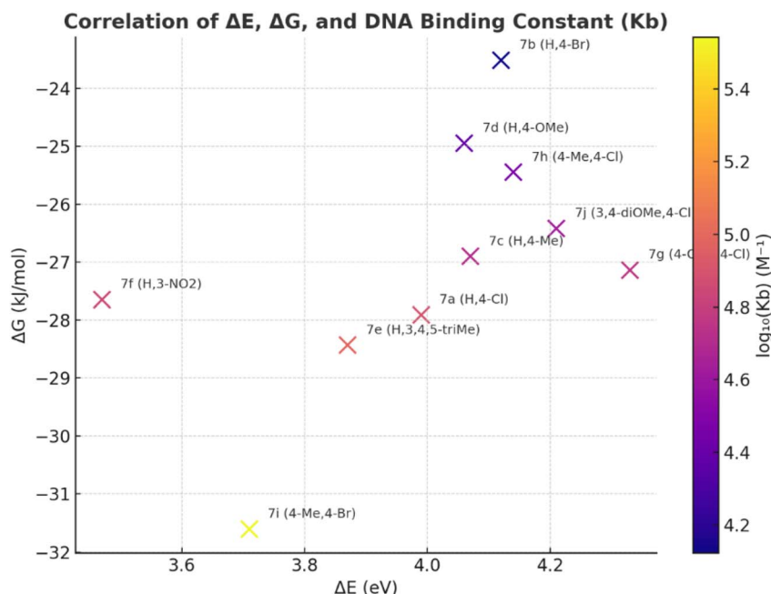
Fig. 7 Qualitative SAR visualization illustrating the influence of electronic substituents on K_b , \Delta E , and \Delta G in the synthesized guanine series.
