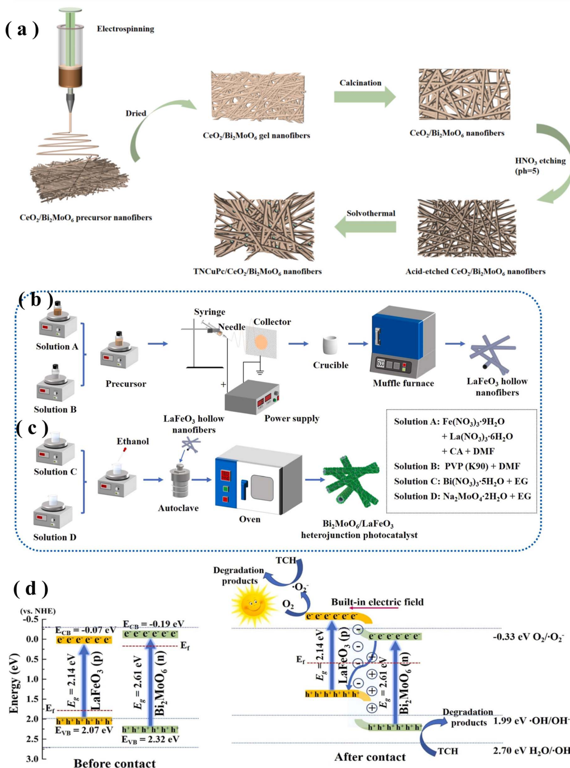
Fig. 3 (a) Schematic diagram of the experimental synthesis of TNCuP/CeO 2 /Bi 2 MoO 6 nanofibers. (b) Illustration of the preparation of LaFeO 3 hollow nanofiber and (c) Bi 2 MoO 6 /LaFeO 3 heterojunction photocatalyst. (d) Illustration of possible mechanisms for charges separation and migration during photocatalytic degradation of TCH over Bi 2 MoO 6 /LaFeO 3 -4. Reproduced from ref. 52 with permission from Elsevier. Copyright 2024.
