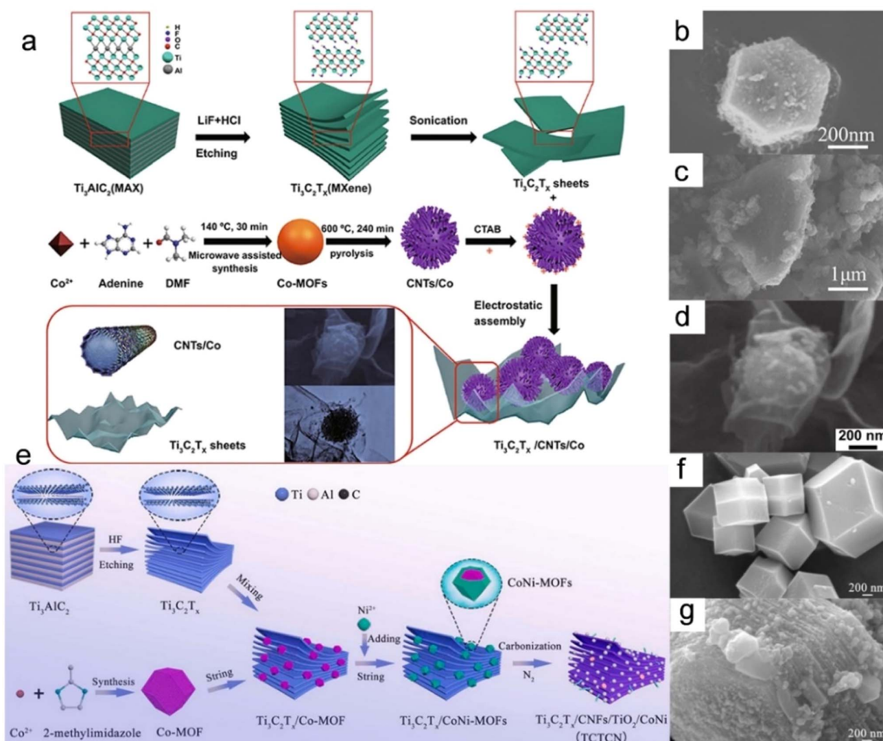
Fig. 7 (a) Synthetic route for \text{Ti}_3\text{C}_2\text{T}_x/\text{CNTs/Co} nanocomposites. SEM images of MXene@Co-CZIF (b), MXene@Ni-CZIF (c), and \text{Ti}_3\text{C}_2\text{T}_x/\text{CNTs/Co} (d). (e) Scheme for the preparation of \text{Ti}_3\text{C}_2\text{T}_x/\text{CNFs/TiO}_2/\text{CoNi} nanocomposites. SEM images of CoNi-MOF (f) and \text{Ti}_3\text{C}_2\text{T}_x/\text{CNFs/TiO}_2/\text{CoNi} nanocomposites (g). (a and d) Reproduced with permission. 234 Copyright 2021, Springer. (b and c) Reproduced with permission. 233 Copyright 2020, American Chemical Society. (e–g) Reproduced with permission. 235 Copyright 2022, Elsevier.
