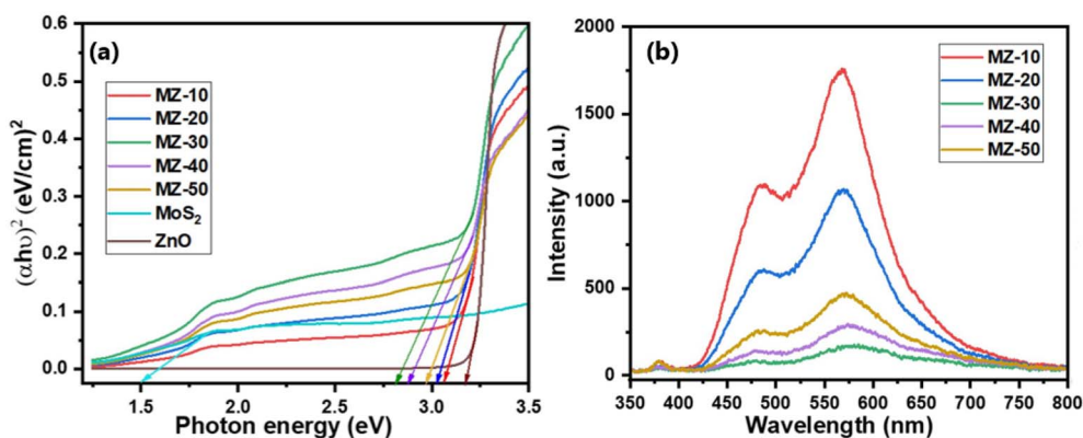
Fig. 34 (a) Bandgap plots of pure \text{ZnO} , \text{MoS}_2 and \text{ZnO}/\text{MoS}_2 hybrid, (b) PL spectra of \text{ZnO}/\text{MoS}_2 hybrid. 426 "Reproduced from ref. 426 with permission from [Elsevier], copyright [2023]."
