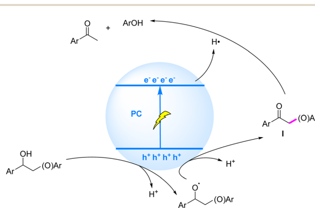
Fig. 8 Mechanisms of C–O bond cleavage induced by ketonic intermediates generated via SET.
