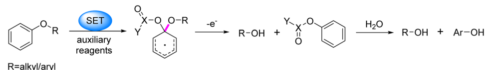
Fig. 2 Dominant pathways of C–C and C–O bond cleavage in lignin under photocatalytic conditions.
