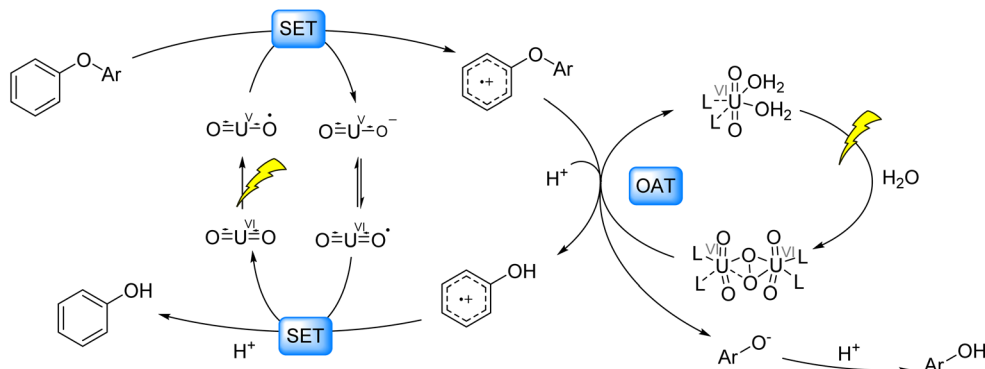
Fig. 13 Photocatalytic cleavage of C–O bonds in 4-O-5 models.
