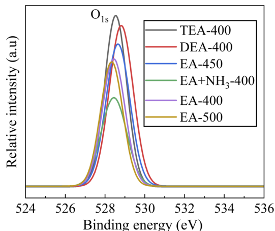
Fig. 7 O 1s XPS spectra of nitrogen-doped \text{TiO}_2 samples, showing characteristic binding energy peaks corresponding to different oxygen chemical environments.
