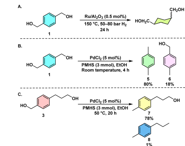
Fig. 3 (A) Synthesis of 1,4-cyclohexanedimethanol ( cis/trans mixture) from 1,4-benzenedimethanol using Ru/Al 2 O 3 catalyst. (B) Hydrodeoxygenation of 1,4-benzenedimethanol using PdCl 2 and polymethylhydrosiloxane (PMHS). (C) Hydrodeoxygenation of 3-(4-(hydroxymethyl)phenyl)propan-1-ol ( 3 ) using PdCl 2 and polymethylhydrosiloxane (PMHS).
