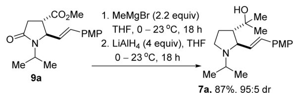
Scheme 1 Synthesis of vicinally functionalized allylic primary pyrrolidinols.
