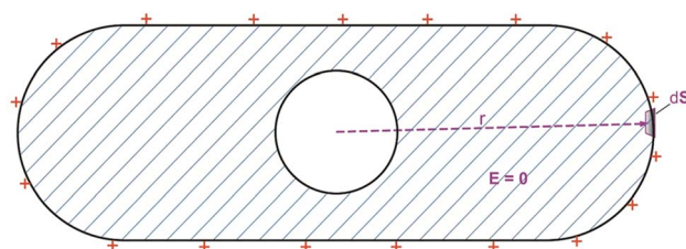
Fig. 5 Closed Gaussian surface inside a volume of conducting materials showing a common physical phenomenon: in a conductor at static equilibrium, all the (extra) electric charge resides on the surface of the conductor. 69
