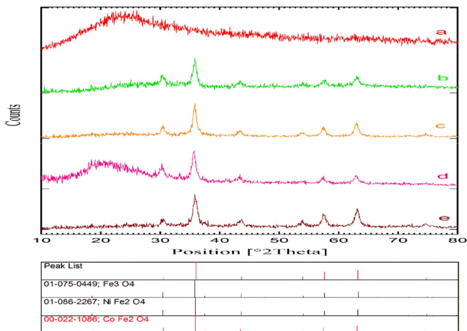
Fig. 3 The XRD patterns of carbon spheres (a), Fe 3 O 4 @carbon nanospheres (b), Co–Ni/Fe 3 O 4 @carbon nanospheres (c), SiO 2 @Co–Ni/Fe 3 O 4 @carbon nanosphere (d), Co–Ni/Fe 3 O 4 @MMSHS (e).
