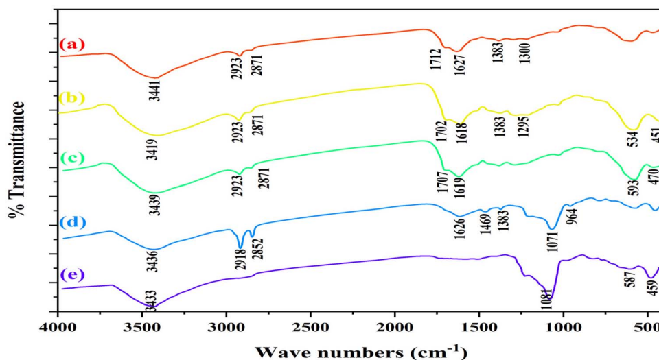
Fig. 2 The FT-IR spectra of carbon spheres (a), Fe 3 O 4 @carbon nanospheres (b), Co–Ni/Fe 3 O 4 @carbon nanospheres (c), SiO 2 @Co–Ni/Fe 3 O 4 @carbon nanosphere (d), Co–Ni/Fe 3 O 4 @MMSHS (e).
