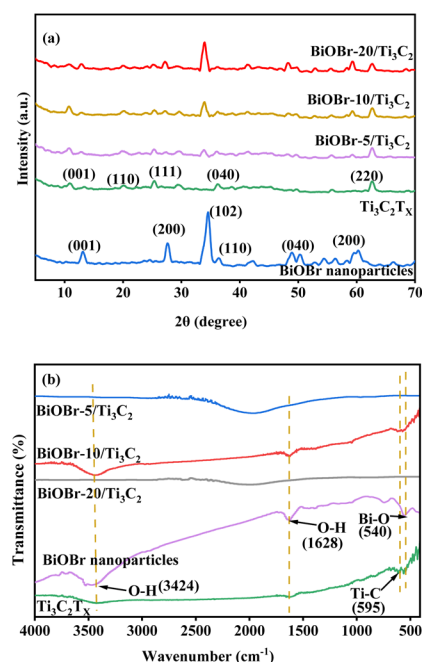
Fig. 2 (a) XRD patterns and (b) FT-IR spectra of BiOBr, \text{Ti}_3\text{C}_2\text{T}_x and BiOBr- x / \text{Ti}_3\text{C}_2\text{T}_x .
