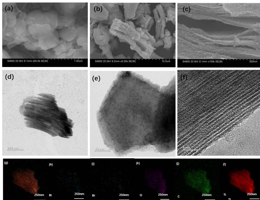
Fig. 1 SEM images of (a) BiOBr, (b) \text{Ti}_3\text{C}_2\text{T}_x and (c) BiOBr-10/ \text{Ti}_3\text{C}_2\text{T}_x ; (d) TEM and magnified TEM (e) images of BiOBr-10/ \text{Ti}_3\text{C}_2\text{T}_x ; (f) HRTEM image of BiOBr-10/ \text{Ti}_3\text{C}_2\text{T}_x ; elemental mapping images of (g) overall distribution, (h) Bi, (i) Br, (j) C, (k) O and (l) Ti in BiOBr-10/ \text{Ti}_3\text{C}_2\text{T}_x .
