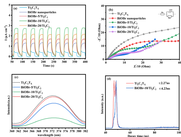
Fig. 4 (a) Transient photocurrent density, (b) Nyquist plots, (c) PL spectra and (d) TRPL spectra of \text{Ti}_3\text{C}_2\text{T}_x , BiOBr and BiOBr- x/\text{Ti}_3\text{C}_2\text{T}_x .
