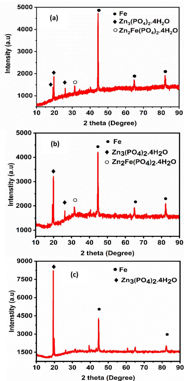
Fig. 6 XRD pattern of zinc phosphate coating corresponding to (a) ZnP, (b) ZnP-0.6CO and (c) ZnP-0.3COCO.
