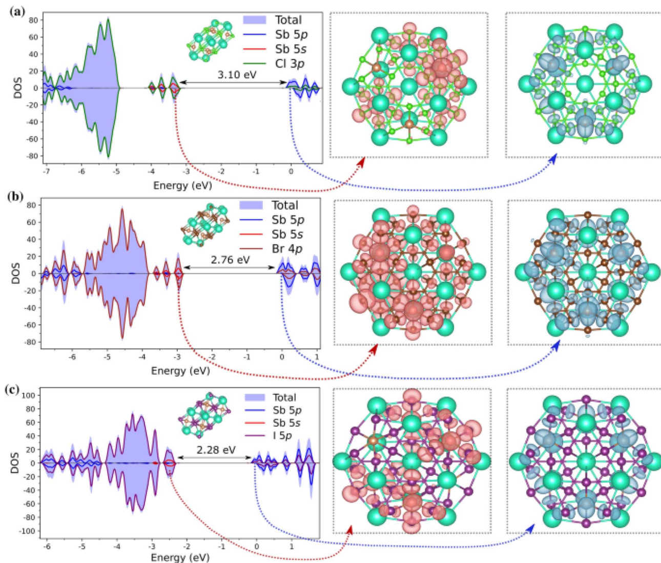
Fig. 8 Partial density of states (PDOS) and frontier molecular orbitals for \text{Cs}_{13}\text{Sb}_6\text{X}_{30} clusters, where \text{X} = \text{Cl}, \text{Br}, \text{and I} . Panels (a), (b), and (c) correspond to the halides Cl, Br, and I, respectively. The total and atomic orbital contributions (Sb 5p, Sb 5s, and halogen p orbitals) to the density of states are shown on the left. The highest occupied molecular orbital (HOMO) and lowest unoccupied molecular orbital (LUMO) distributions are visualized on the right for each composition, with the energy band gaps indicated between the HOMO and LUMO levels. 201
