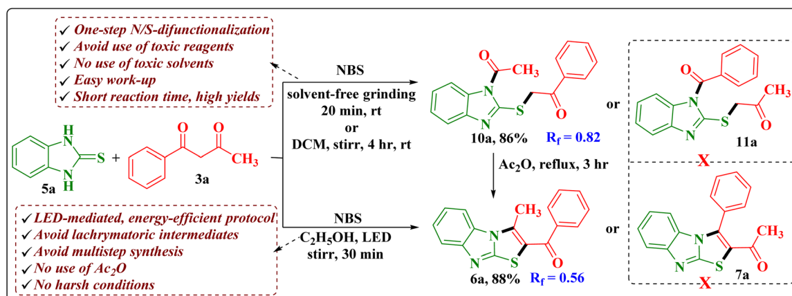
Scheme 2 Synthesis of benzo[4,5]imidazo[2,1- b ]thiazoles.
