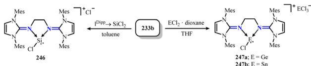
Scheme 87 Synthesis of bis(NHI)-stabilized tetryliumylidenes 246 – 247 .
