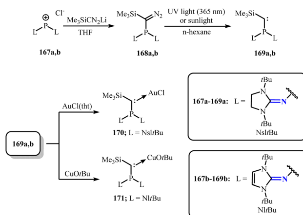
Scheme 65 Synthesis of phosphino(silyl)carbenes 169a and 169b and its reaction with AuCl(tht) (tht = tetrahydrothiophene) and CuOtBu.
