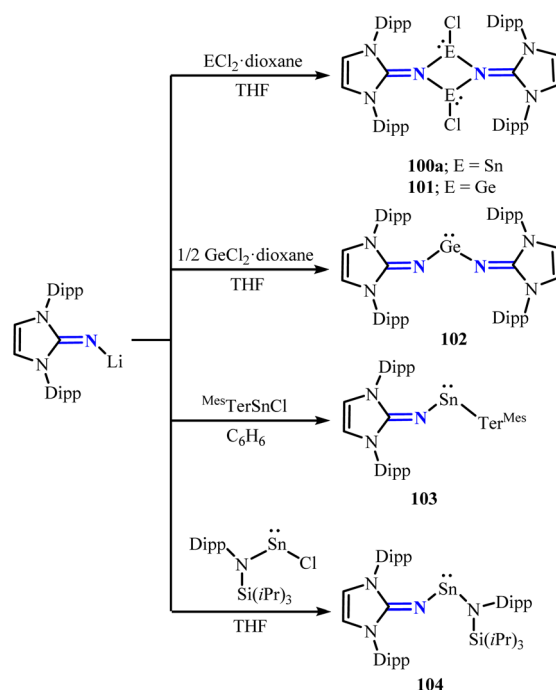
Scheme 41 Synthesis of tetrelenes 100a , 101 – 104 . Mes 3 Ter = 2,6-Mes 2 C 6 H 3 .
