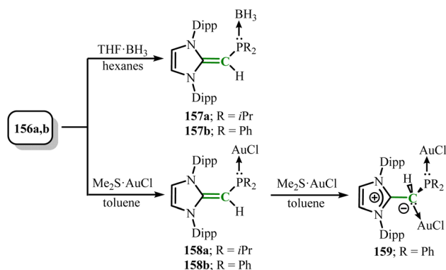
Scheme 62 Reaction of 156a and 156b with BH 3 , Me 2 S·AuCl.
