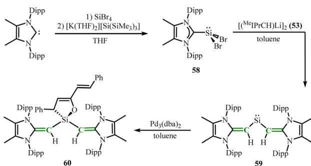
Scheme 24 Synthesis of bicoordinated acyclic silaalkenes 59 and its reaction with [\text{Pd}_3(\text{dba})_2] .
