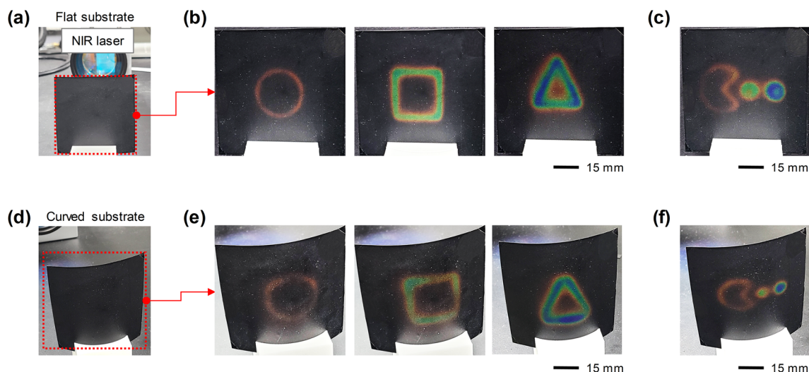
Fig. 5 Images of the light-irradiation-based color-conversion display on flat and curved surfaces. Displays on (a) flat and (d) curved substrates showing (b and e) circular (R), square (G), and triangular (B) images and (c and f) full-color Pac-Man images.
