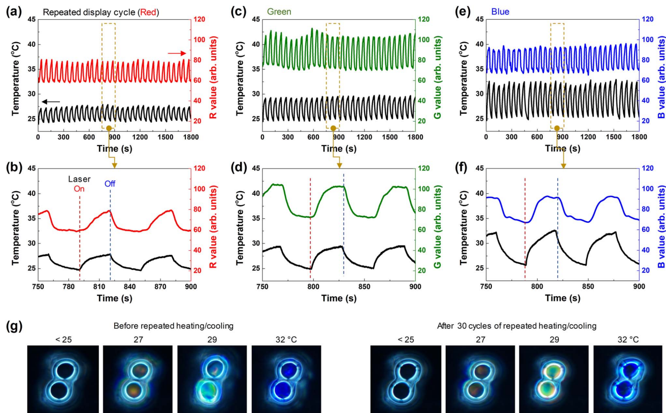
Fig. 4 Repeated RGB color generation by the light-irradiation-based color-conversion display. The on/off time for all the displays was fixed at 30/30 s. Repeated driving characteristics of the (a and b) red (laser power: 25 mW), (c and d) green (laser power: 36 mW), and (e and f) blue (laser power: 56 mW) displays. (g) Optical microscope image of the TLC capsule after 30 cycles of repeated heating/cooling (5/5 min) testing.
