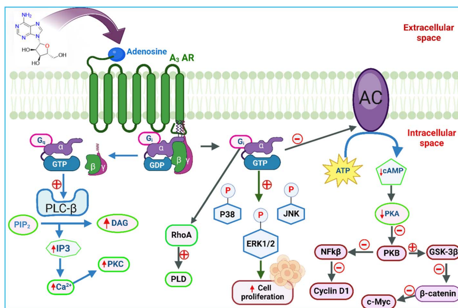
Fig. 6 A 3 adenosine receptors' role in cancer: molecular signalling pathways. ERK1/2 – “Extracellular signal-regulated kinases”, ATP – “Adenosine triphosphate”, PKA – “protein kinase A”, PIP2 – “Phosphatidylinositol 4,5-bisphosphate”, FoxP3 – “Forkhead box P3”, GSK-3 \beta – “Glycogen synthase kinase-3 \beta ”, IP3 – “Inositol trisphosphate”, cAMP – “Cyclic adenosine monophosphate”, JNK – “c-Jun N-terminal kinases”, DAG – “Diacylglycerol”, PKC – “Protein kinase C”, PKB – “Protein kinase B”, RhoA – “Ras homolog family member A” and NF \kappa B – “Nuclear factor kappa-light-chain-enhancer of activated B cells”. The figure was created in BioRender. Deb, P. (2025).
