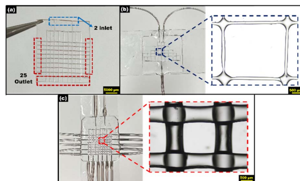
Fig. 6 (a) Fabricated 2-inlet–25-outlet mesh design (microchannel diameter: 370 μm). (b) Fabricated device featuring a tree-shaped design (microchannel diameter: ~180 μm). (c) Fabricated device with a microchannel diameter of ~700 μm.
