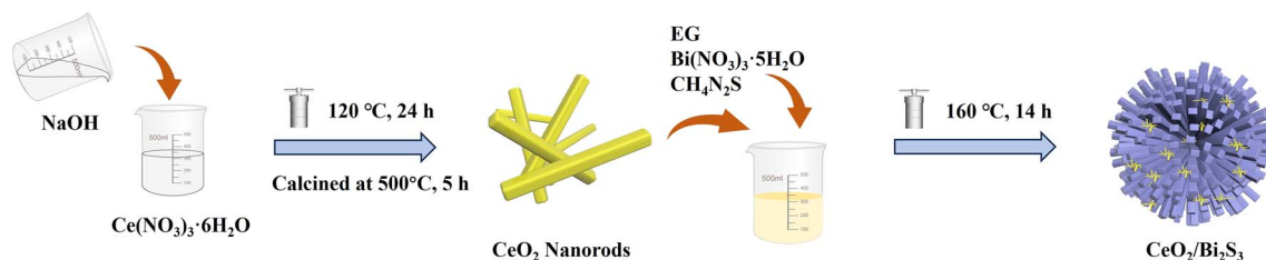
Scheme 1 Schematic illustration of the synthesis of \text{CeO}_2/\text{Bi}_2\text{S}_3 photocatalysts.
