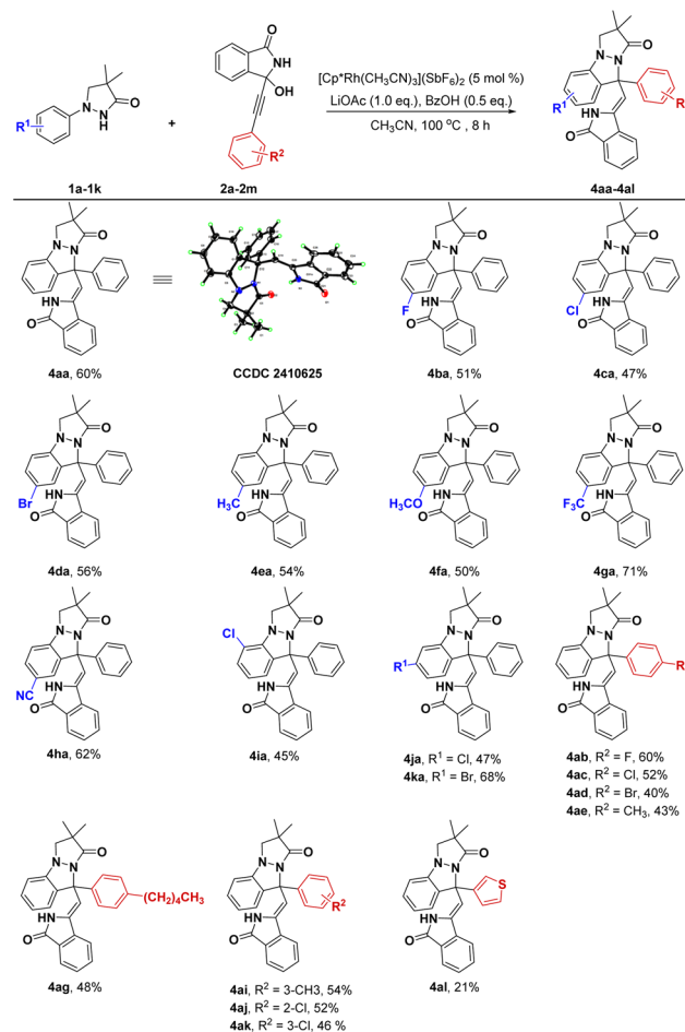
Scheme 3 The investigation of substrate scope for the synthesis of 4 . General reaction conditions (condition B): 1 (0.24 mmol), 2 (0.2 mmol), [Cp*Rh(CH 3 CN) 3 ](SbF 6 ) 2 (5 mol%), LiOAc (0.2 mmol), BzOH (0.1 mmol) in MeCN (4.0 mL) at 100 °C under air for 8 h, isolated yields.
