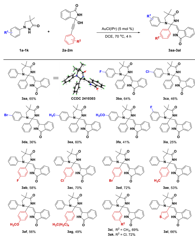
Scheme 2 The investigation of substrate scope for the synthesis of 3 . General reaction conditions (condition A): 1 (0.24 mmol), 2 (0.2 mmol), AuCl(IPr) (5 mol%) in DCE (4.0 mL) at 70 °C under air for 4 h, isolated yields.
