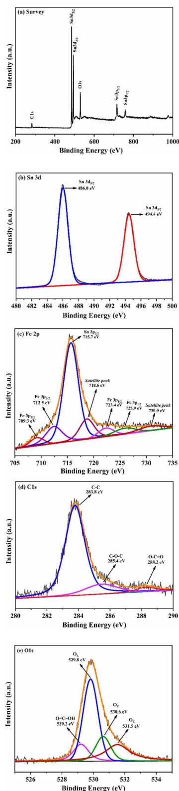
Fig. 4 (a) XPS survey spectrum, (b) Sn 3d, (c) Fe 2p, (d) C 1s and (e) O 1s core level XPS spectrum of S3 nanocomposite.
