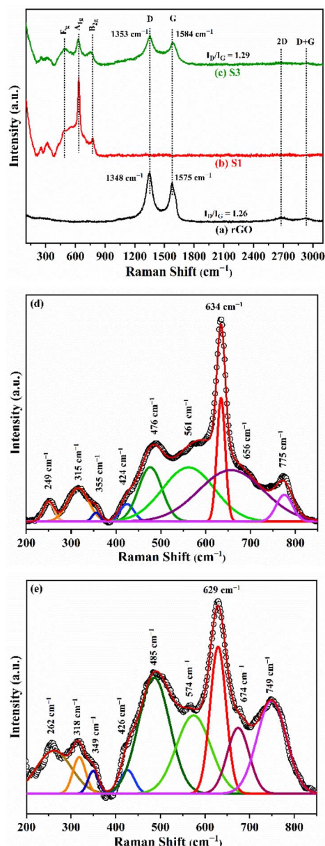
Fig. 5 (a) Raman spectra of rGO, (b) S1, and (c) S3, (b and d) deconvoluted Raman spectra of S1 and (c and e) S3 nanocomposite in the wavenumber range 200–850 cm -1 .
