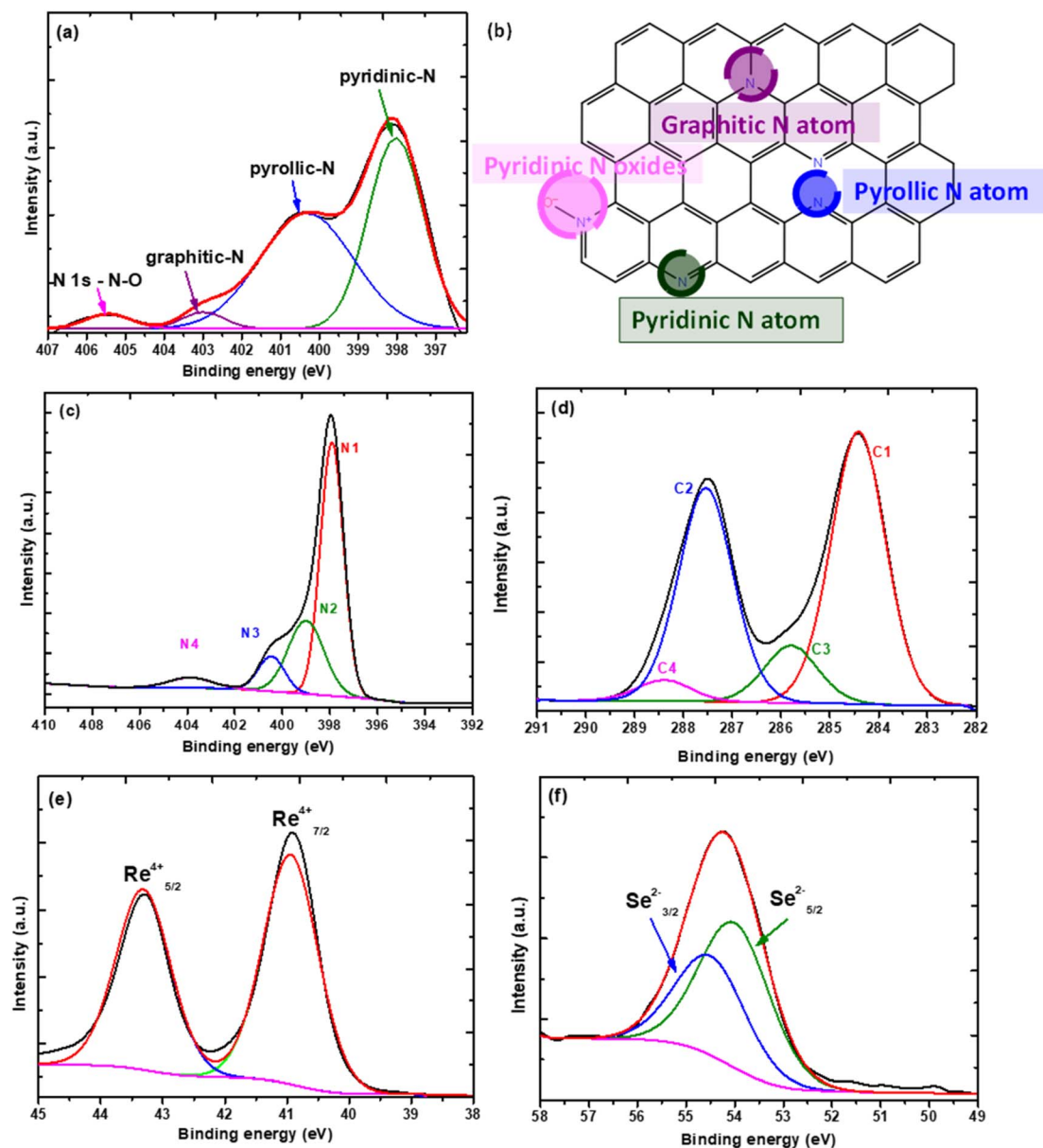
Fig. 2 (a) Deconvoluted XPS spectrum of the N1s peak for N-rGO. (b) Graphical representation of the types of nitrogen defects introduced. (c) Deconvoluted N1s peak of g\text{-C}_3\text{N}_4 . (d) Deconvoluted C1s peak of g\text{-C}_3\text{N}_4 . (e) High-resolution XPS spectrum of Re. (f) High-resolution XPS spectrum of Se.
