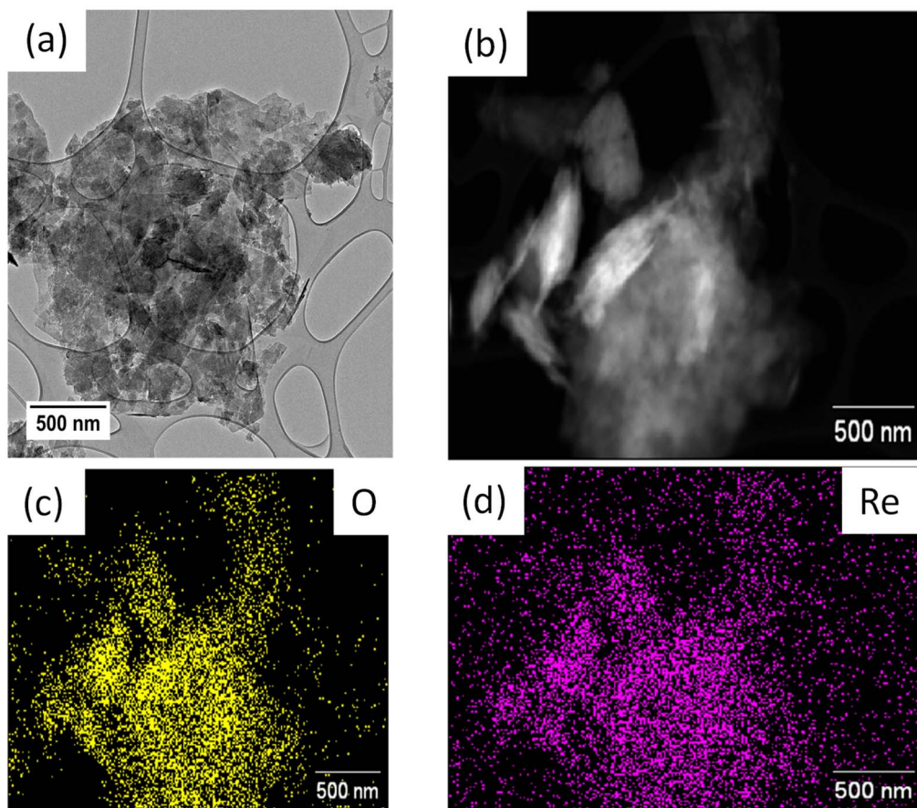
Fig. 5 (a) Sheetlike structure of rGO after introduction of Re monomer. (b) Grey image of rGO-ReO 4 2- . Elemental mapping of (c) oxygen and (d) rhenium.
