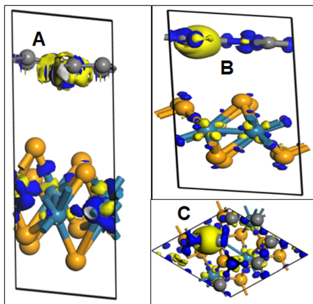
Fig. 12 The three-dimensional (3D) charge density differences of (A) ReSe 2 -rGO heterostructure, (B) side view of ReSe 2 -N-rGO heterostructure and (C) top view of ReSe 2 -N-rGO heterostructure. The yellow and blue colours represent the accumulation and depletion of electrons, respectively.
