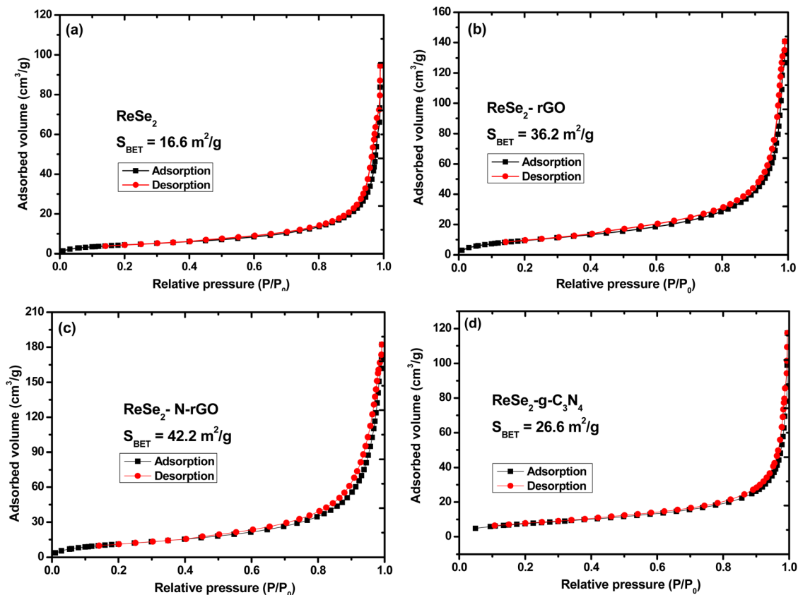
Fig. 9 Adsorption-desorption isotherms of (a) \text{ReSe}_2 , (b) \text{ReSe}_2 -rGO, (c) \text{ReSe}_2 -N-rGO, and (d) \text{ReSe}_2 -g- \text{C}_3\text{N}_4 .
