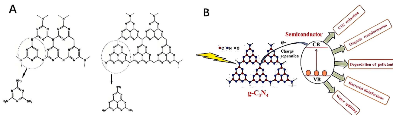
Fig. 2 Photocatalytic reactions of carbon–nitride-based materials. (A) g\text{-C}_3\text{N}_4 has two structures, namely the triazine (a) and the tri- s -triazine. 17 (B) Mechanism and application of g\text{-C}_3\text{N}_4 photocatalytic reaction. 18
