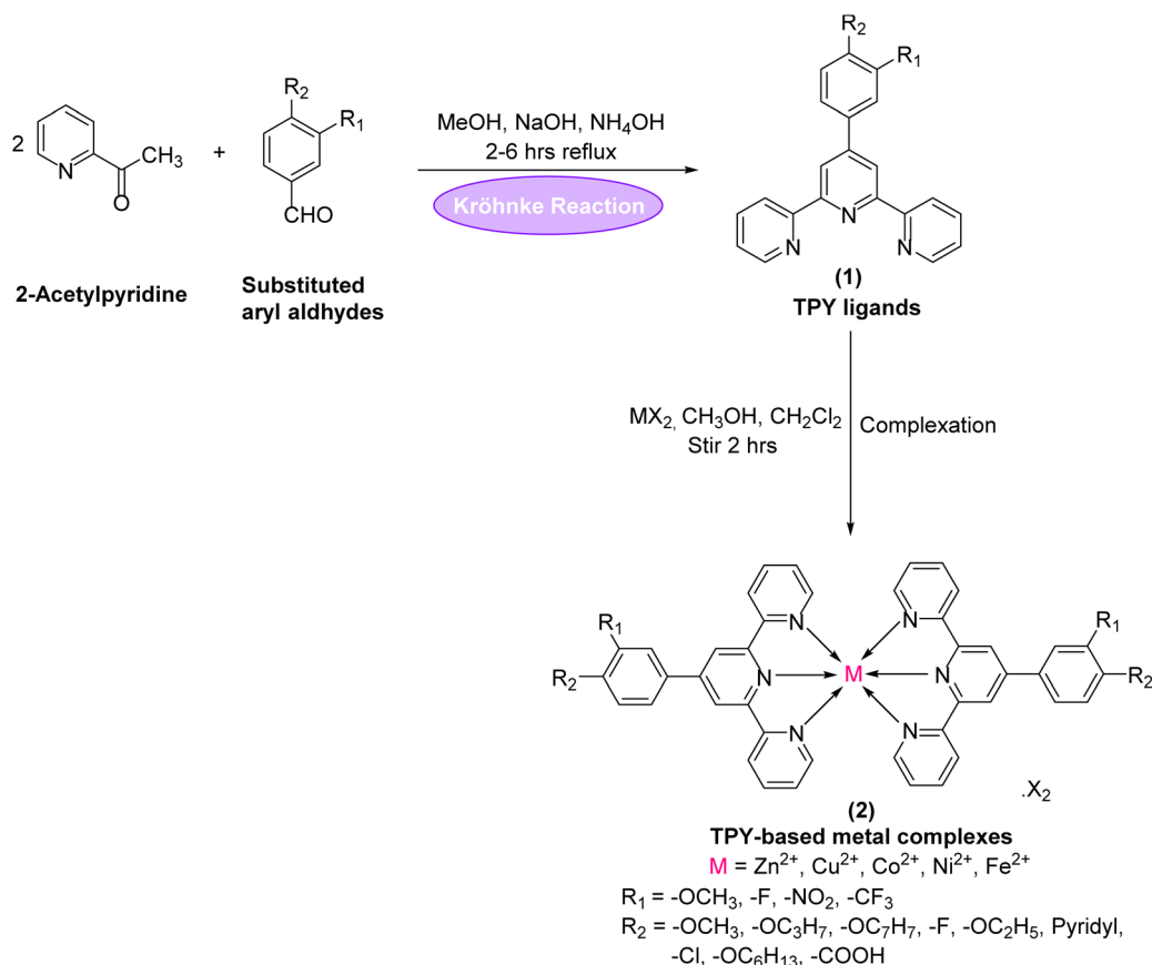
Scheme 1 Synthesis of TPY ligands ( \text{L}_1 – \text{L}_{11} ) and their metal complexes ( \text{C}_1 – \text{C}_{20} ).
