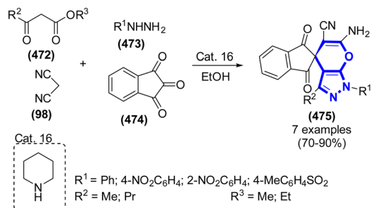
Scheme 127 Synthesis of spiro-pyranopyrazoles and oxa-aza-[3.3.3]propellanes catalyzed by Cat. 16 in ethanol.
