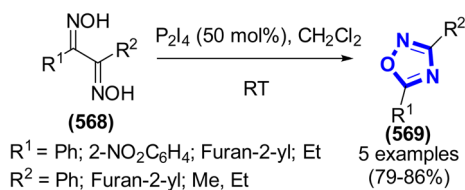
Scheme 151 Synthesis of 1,2,4-oxadiazole derivatives catalyzed by \text{P}_2\text{I}_4 .
