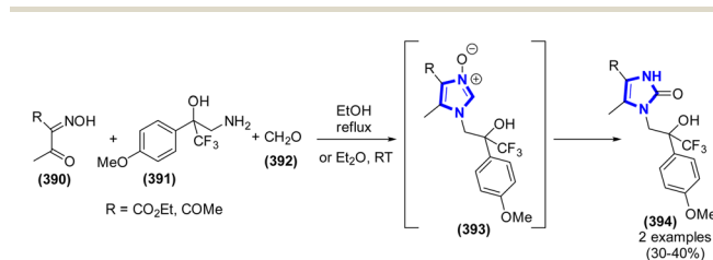
Scheme 104 Synthesis of imidazolone frameworks in ethanol.
