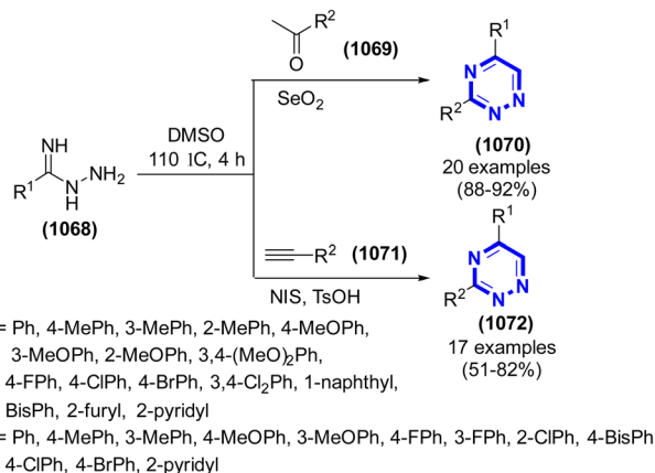
Scheme 297 Synthesis of 1,2,4-triazine catalyzed by SeO 2 or NIS-TsOH systems.
