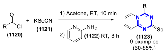
Scheme 309 Synthesis of 2H-pyrido[1,2-a][1,3,5]triazine-2-selenones.
