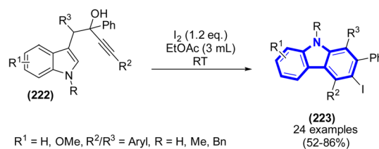
Scheme 60 Synthesis of 3-iodocarbazoles catalyzed by I 2 .
