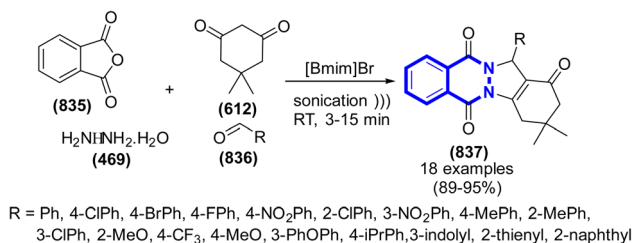
Scheme 237 Synthesis of phthalazinetriones catalyzed by 1-butyl-3-methylimidazolium bromide.
