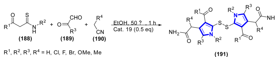
Scheme 51 Synthesis of pyrrole analogs using Cat. 19.
