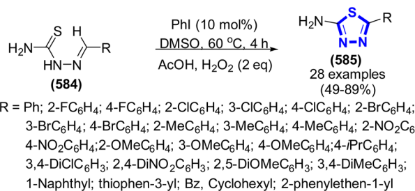
Scheme 157 Synthesis of 2-amino-1,3,4-thiadiazole catalyzed by PhI.
