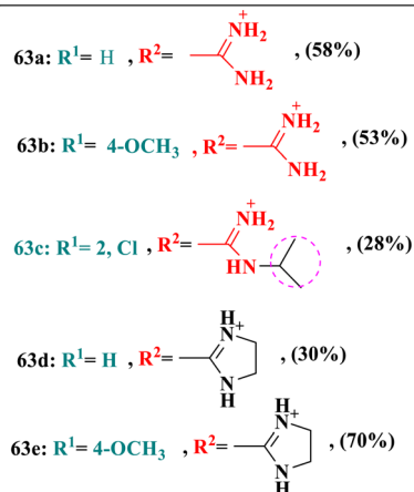
Fig. 6 Structures of benzimidazole-triazole hybrids with amidino moieties 63a–e , synthesized for evaluation against Gram-positive and Gram-negative bacteria.
