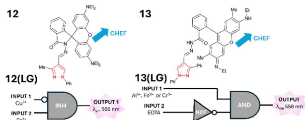
Fig. 14 Rhodamine-pyrazole 12 and 13 and their application as logic gates 12(LG) and 13(LG) . 38,39
