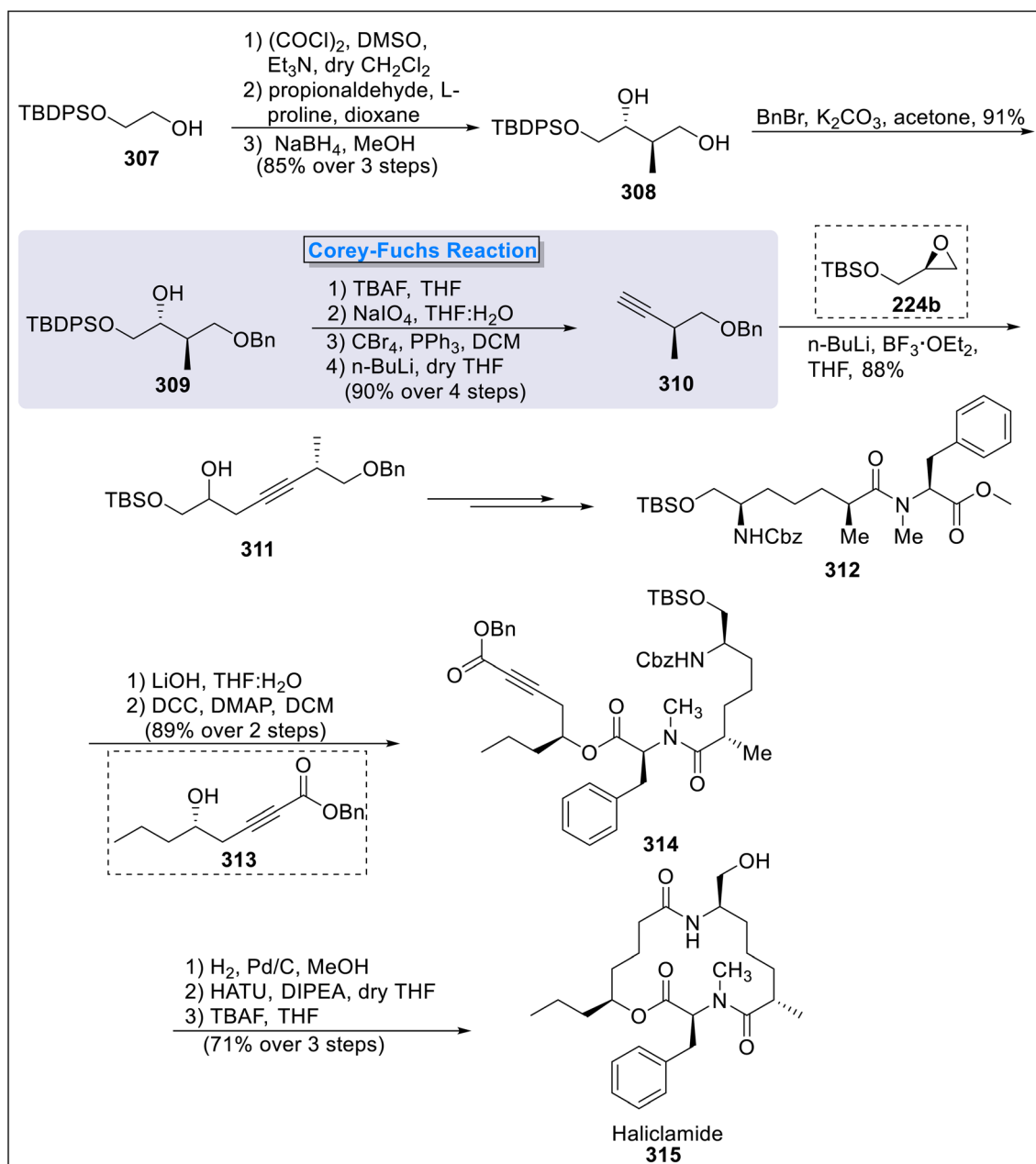
Scheme 31 Total synthesis of haliclamide 315 by Galawat and coworkers.
