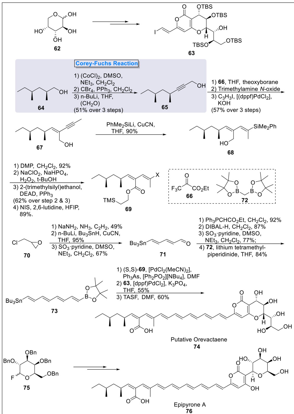
Scheme 7 Total synthesis of putative orevactaene 74 &amp; epipyron A 76 by Preindl and coworkers.
