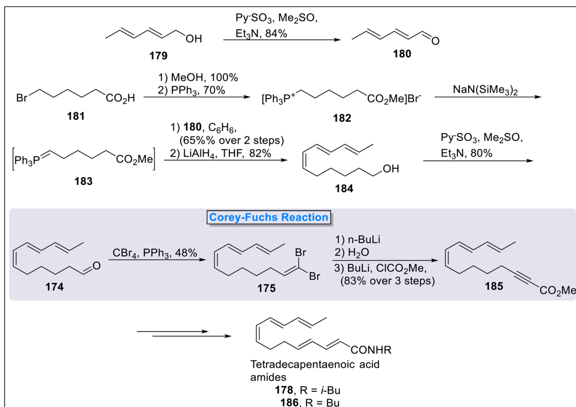
Scheme 17 Total synthesis of tetradecapentaenoic acid derivatives 178 & 186 by Kolodiazna & Kolodiazny.
