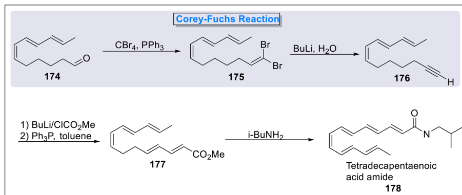
Scheme 16 Total synthesis of tetradecapentaenoic acid amide 178 by Kolodiazna & Kolodiazny.
