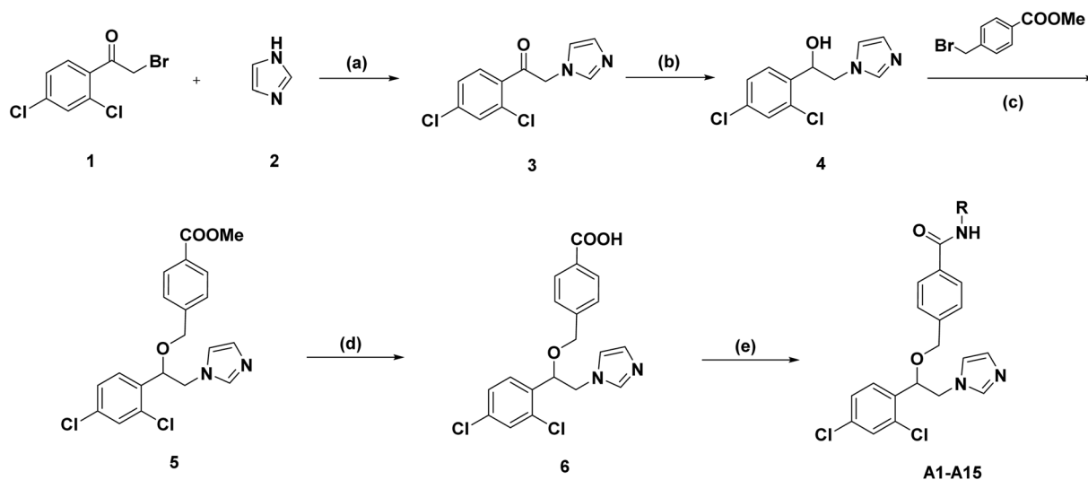
Scheme 1 Synthetic route of target compounds A01–A15 . Reagents and conditions: (a) Et 3 N, MeOH, 65 °C, 4 h, 90%; (b) NaBH 4 , MeOH, 25 °C, 2 h, 80%. (c) NaH, tetrahydrofuran, 70 °C, 4 h, 65.5%; (d) KOH, MeOH, reflux, 1 h (without purification); (e) R-NH 2 , DCM, DMAP, EDCI, 25 °C, 1 h.
