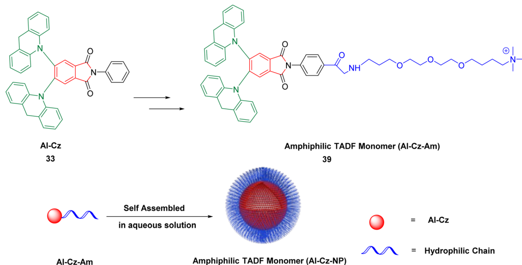
Fig. 17 Structure of amphilphilic TADF monomer 39 and the synthesis of TADF nanoprobe AI-Cz-NP. Reproduced from ref. 163 with permission from the Royal Society of Chemistry.
