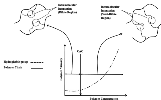
Fig. 9 Evolution of viscosity in hydrophobically associating polymers across the critical aggregation concentration threshold. This figure demonstrates the viscosity changes of hydrophobically associating polymers before and after reaching the critical aggregation concentration (CAC). 67
