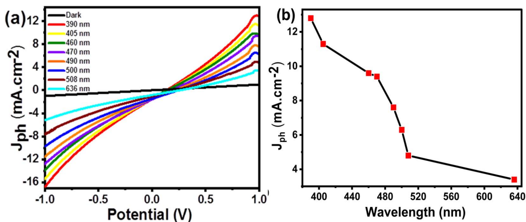
Fig. 7 (a) The relationship between the photocurrent values and the voltage in the presence of several wavelengths and (b) the correlation of J_{ph} – \lambda at +1 V for KI:CTC/CuO photodetector.
