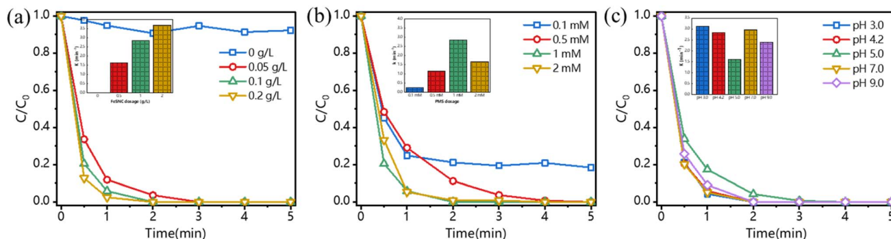
Fig. 4 Kinetic curves of BPA degradation and apparent rate constant ( k obs ) by FeSNC-PMS system with (a) different catalyst dosage, (b) different PMS concentration and (c) different initial pH. Experimental conditions: [BPA] 0 = 20 mg L -1 , [PMS] 0 = 1 mM, [catalyst] 0 = 0.10 g L -1 , initial pH 4.2.
