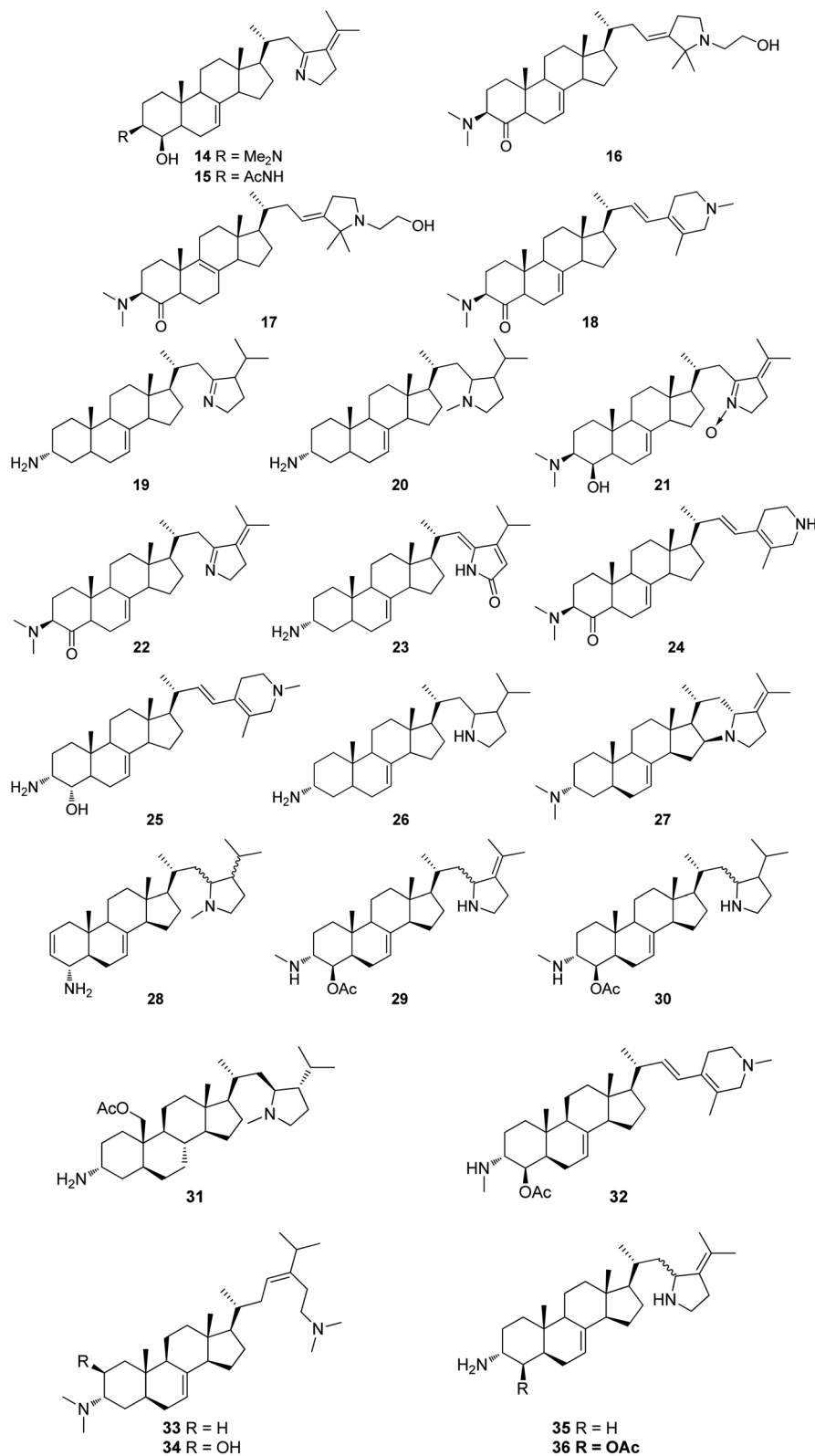
Fig. 3 Reported plakinamines 14–36.
