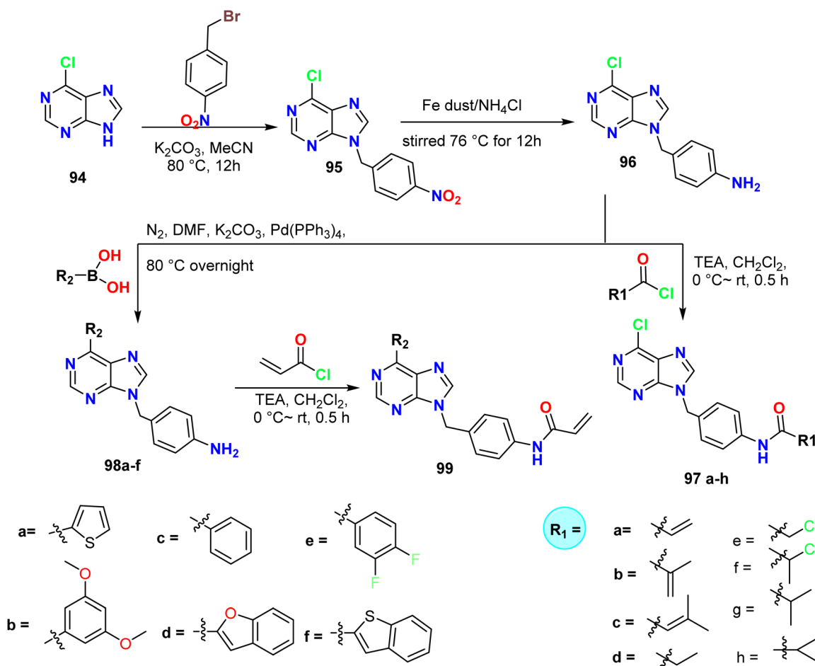
Scheme 25 Synthesis of 9-substituted-9H-purine derivatives 97a–h , 98a–f , and 99a–f through alkylation reactions.
