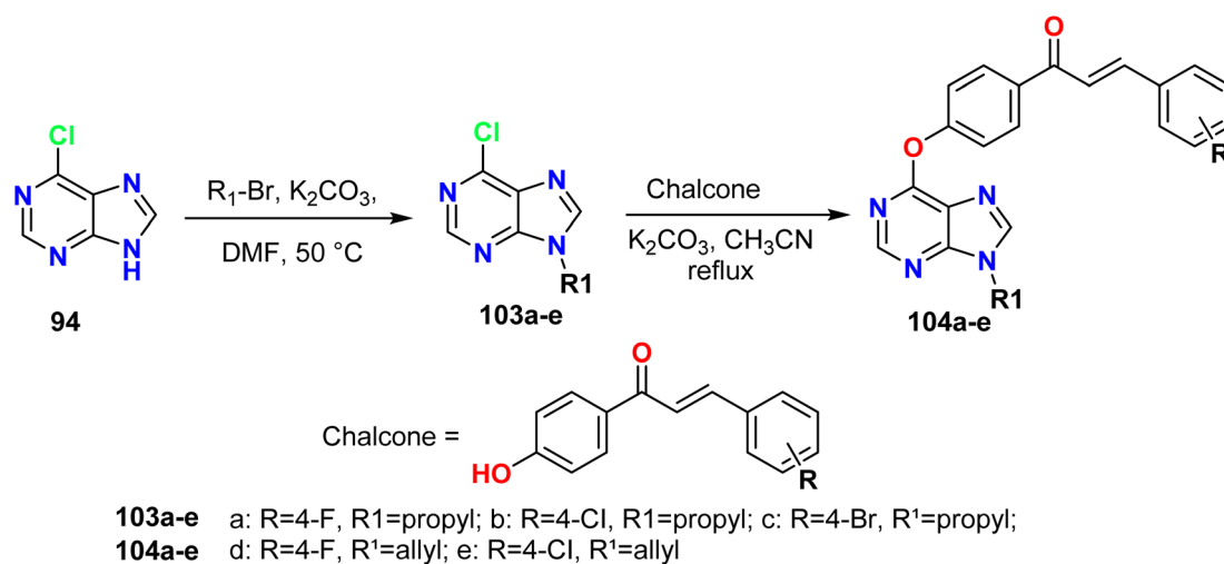
Scheme 27 Synthesis of 6,9-disubstituted purine derivatives 104a–e from 6-chloro-9H-purine.
