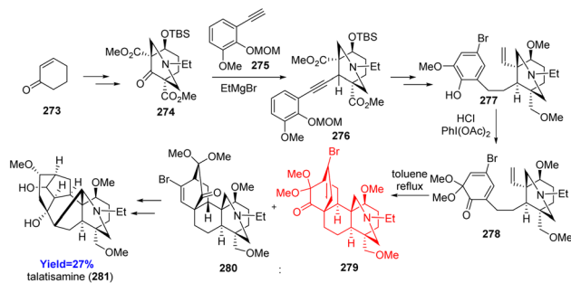
Scheme 35 Total synthesis of talatisamin (281). 84
