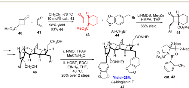
Scheme 7 Total synthesis of kingianin F ( 47 ). 35
