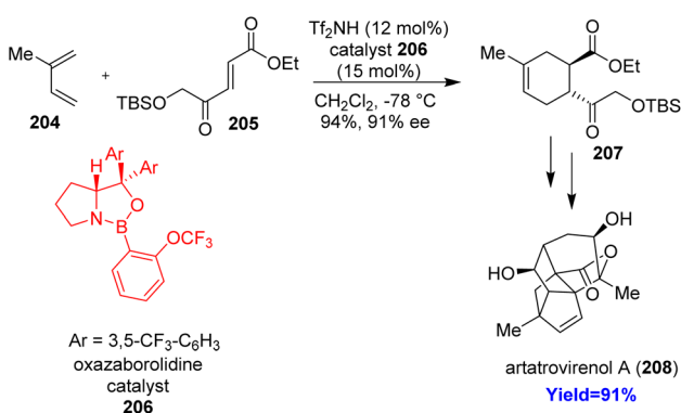
Scheme 26 Total synthesis of artatrovireno A (208). 63
