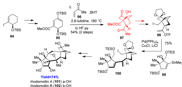
Scheme 13 Total syntheses of rhodomollins A ( 101 ) a-OH rhodomollin B ( 102 ) b-OH. 43
