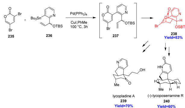
Scheme 30 Stille coupling between ( 235 ) and ( 236 ) accompanied with IMDA reaction produced ( 238 ) which further can be converted to the lycopoladine A ( 239 ) and (–)-lycopoloserramine R ( 240 ). 72
