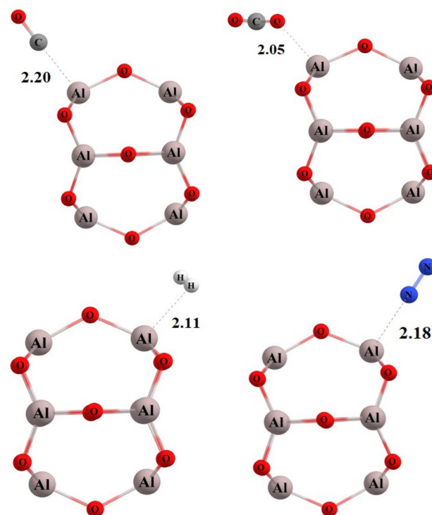
Fig. 4 Optimized structures of gas molecules \text{CO} , \text{CO}_2 , \text{H}_2 , and \text{N}_2 adsorbed on the outer surface of the \text{Al}_8\text{O}_{12} cluster. Calculations were performed at the \omega\text{B97XD/Def2-TZVP} level of theory. Bond lengths are presented in Å.
